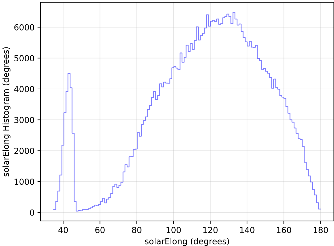
roll_pause_mjdp180_v3.4_10yrs All sky z band: solarElong Histogram
