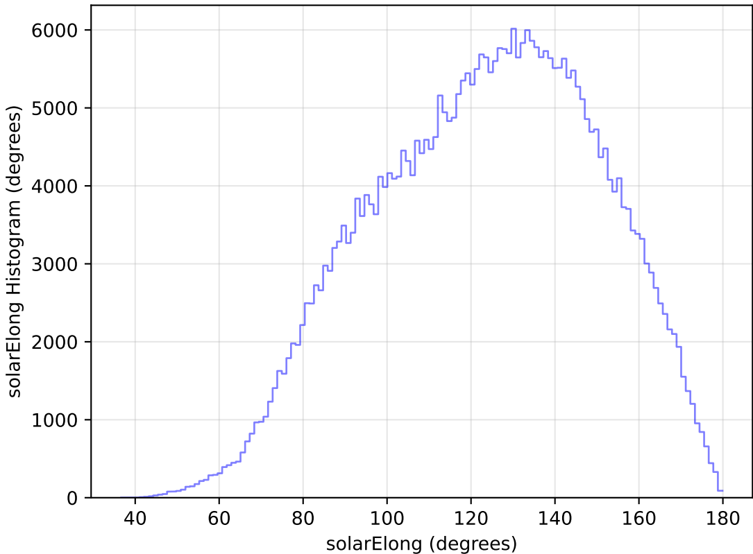
roll_pause_mjdp180_v3.4_10yrs All sky y band: solarElong Histogram
