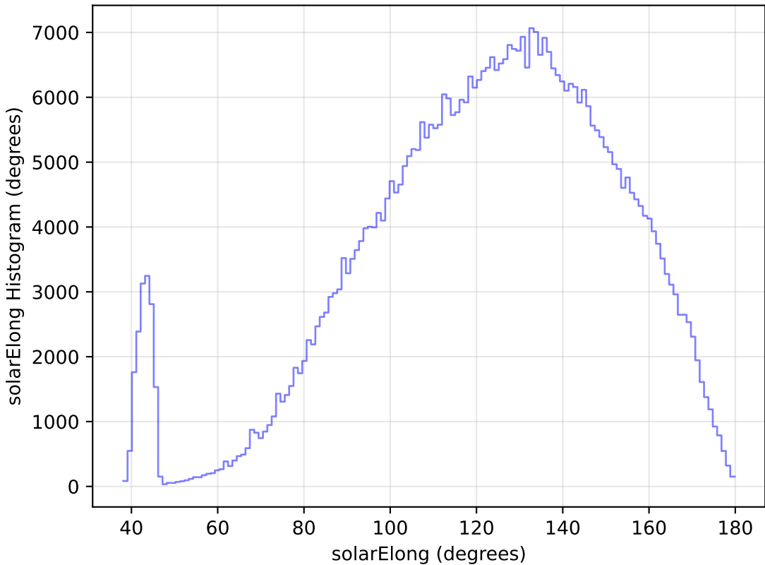
roll_pause_mjdp180_v3.4_10yrs All sky r band: solarElong Histogram
