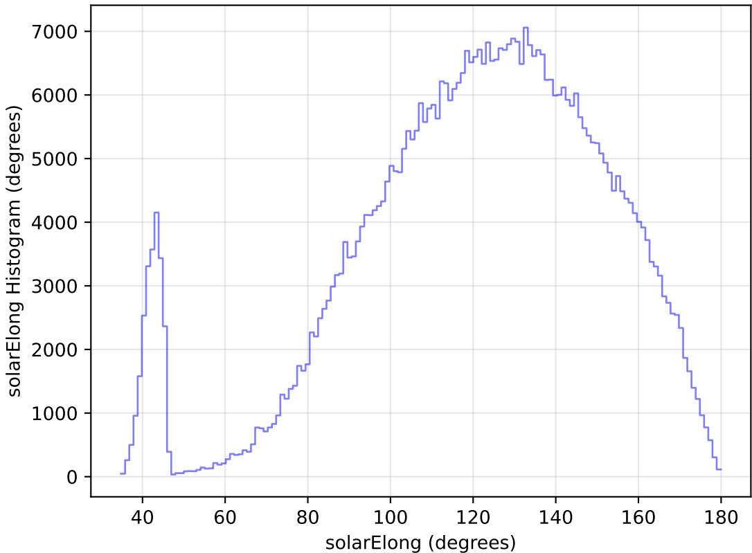
roll_pause_mjdp180_v3.4_10yrs All sky i band: solarElong Histogram
