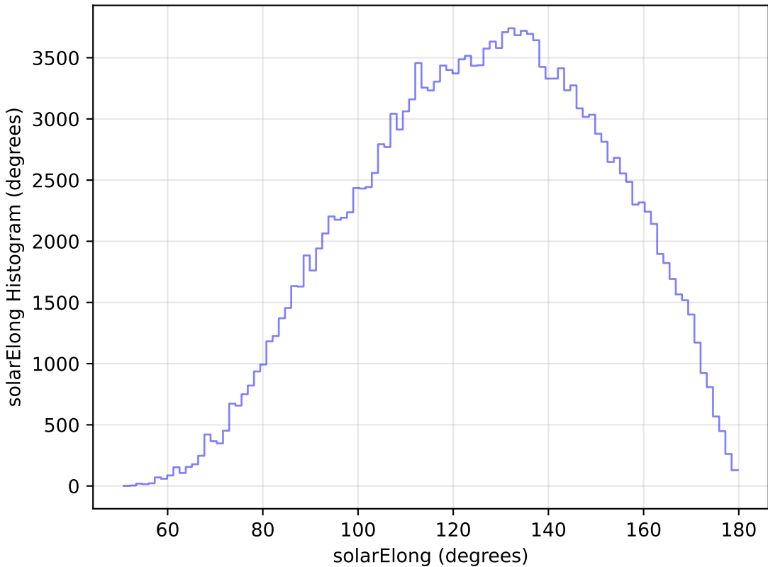
roll_pause_mjdp180_v3.4_10yrs All sky g band: solarElong Histogram
