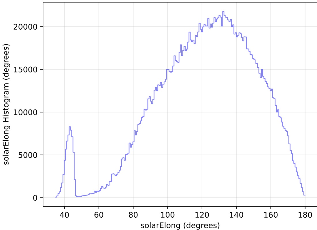
roll_pause_mjdp180_v3.4_10yrs All sky all bands: solarElong Histogram
