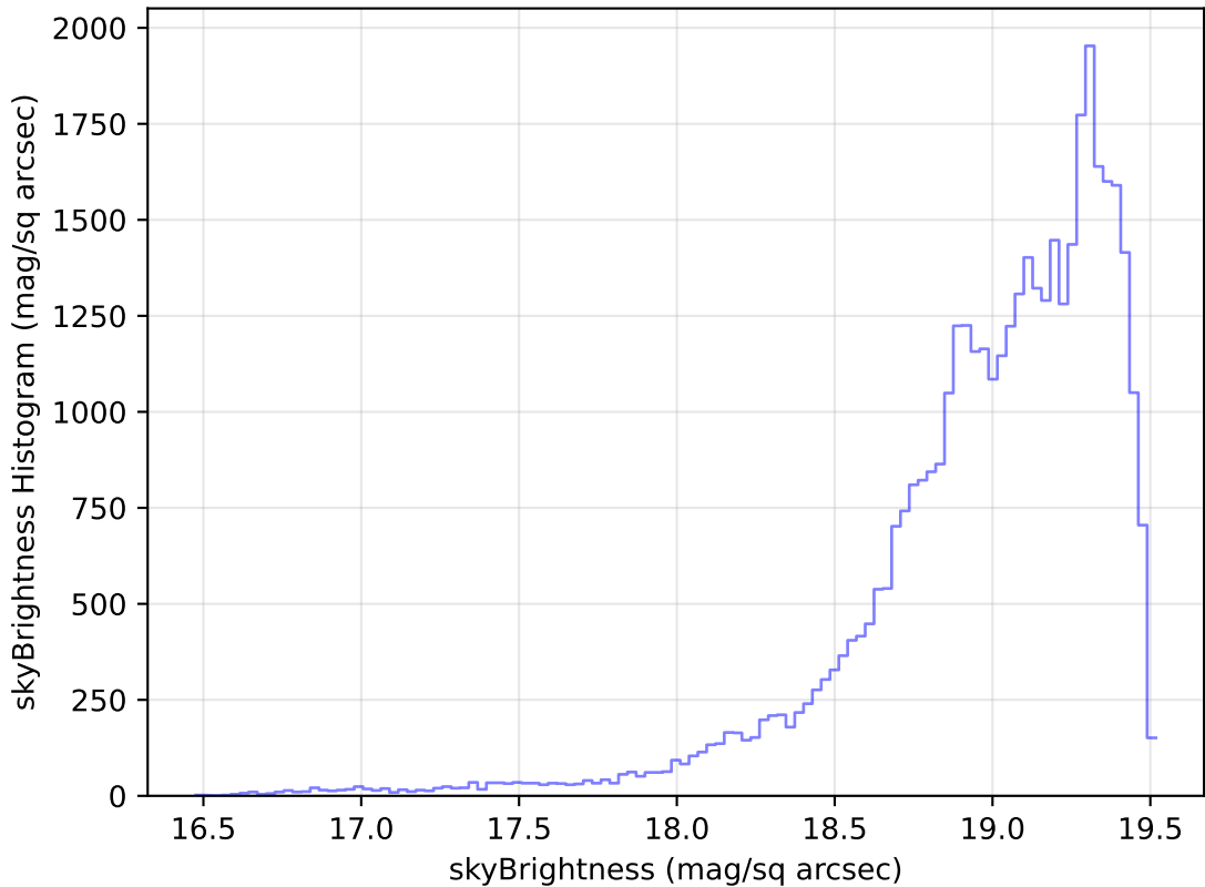
roll_pause_mjdp180_v3.4_10yrs Yr 1 z band: skyBrightness Histogram
