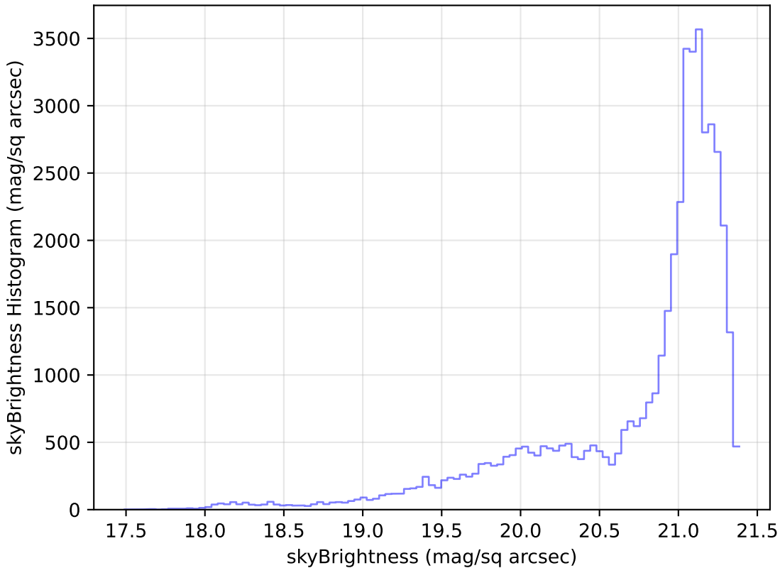
roll_pause_mjdp180_v3.4_10yrs Yr 1 r band: skyBrightness Histogram
