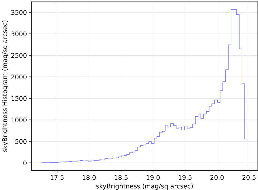
roll_pause_mjdp180_v3.4_10yrs Yr 1 i band: skyBrightness Histogram
