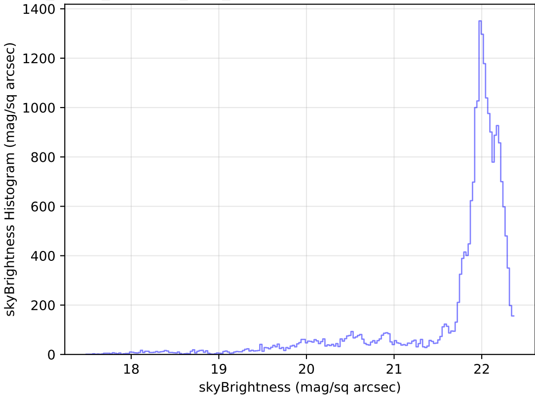
roll_pause_mjdp180_v3.4_10yrs Yr 1 g band: skyBrightness Histogram
