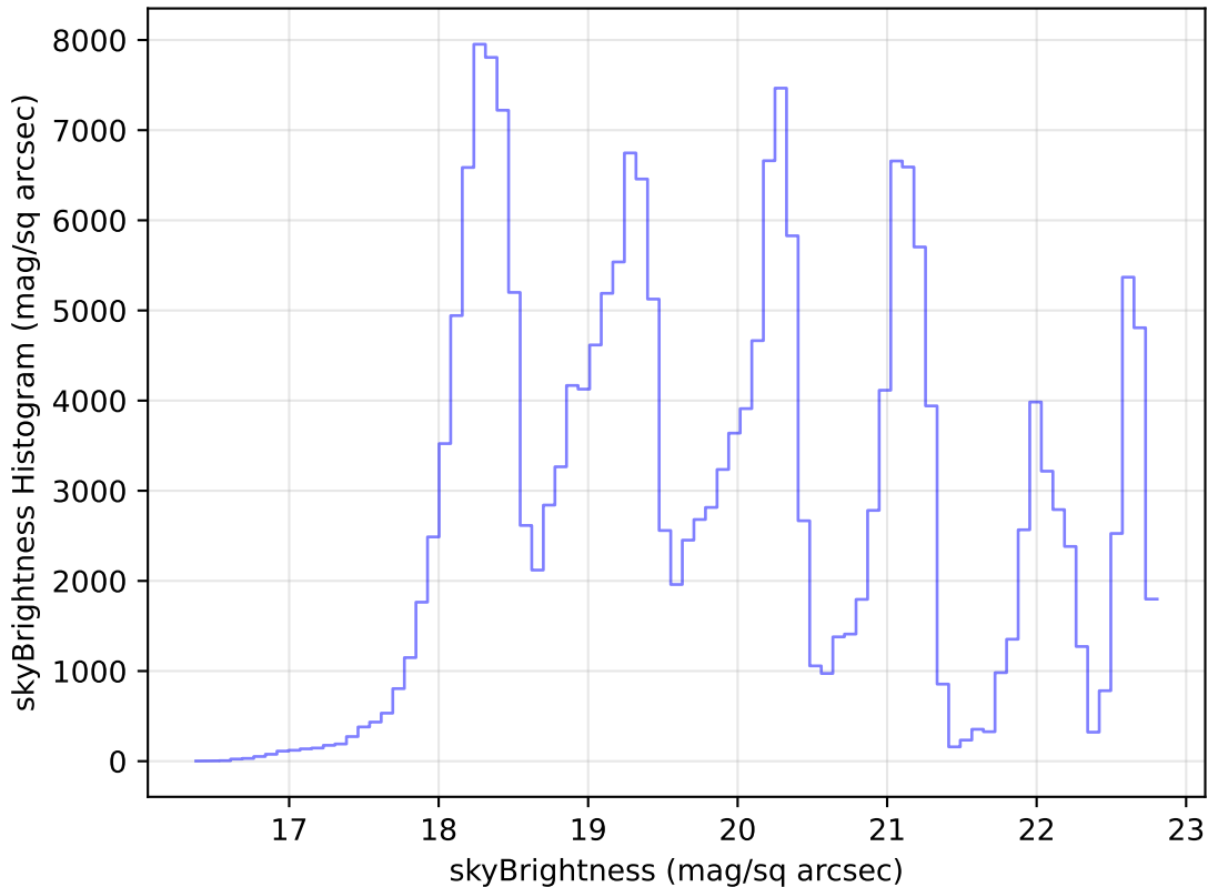
roll_pause_mjdp180_v3.4_10yrs Yr 1 all bands: skyBrightness Histogram
