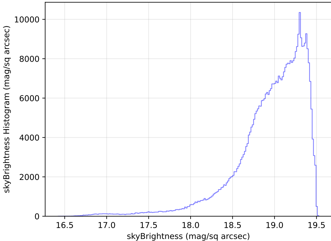
roll_pause_mjdp180_v3.4_10yrs WFD z band: skyBrightness Histogram
