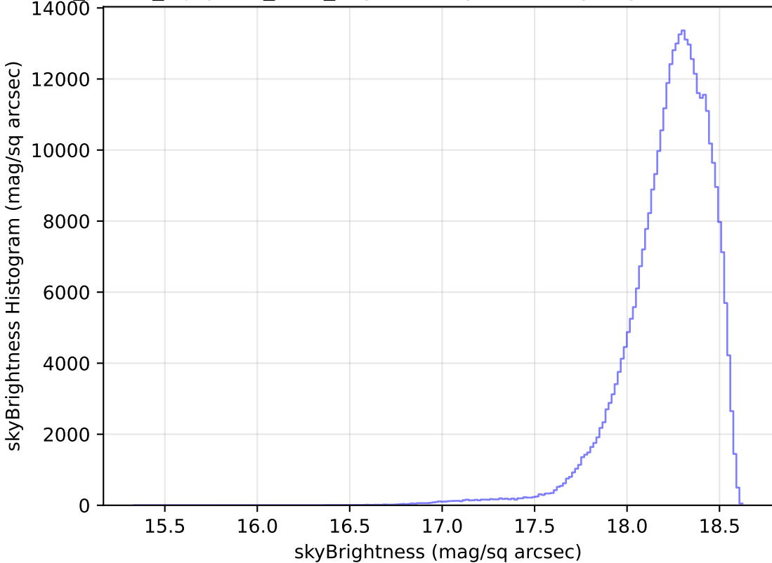
roll_pause_mjdp180_v3.4_10yrs WFD y band: skyBrightness Histogram
