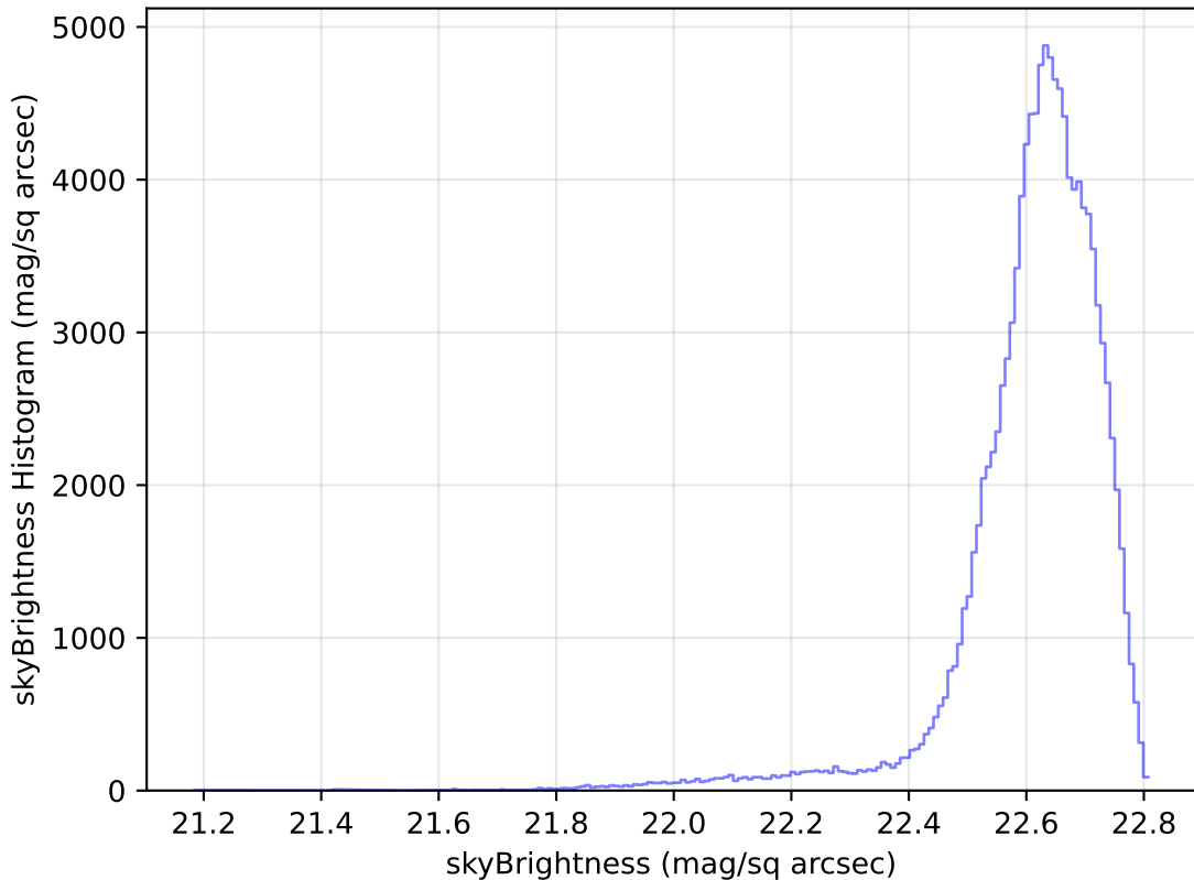
roll_pause_mjdp180_v3.4_10yrs WFD u band: skyBrightness Histogram
