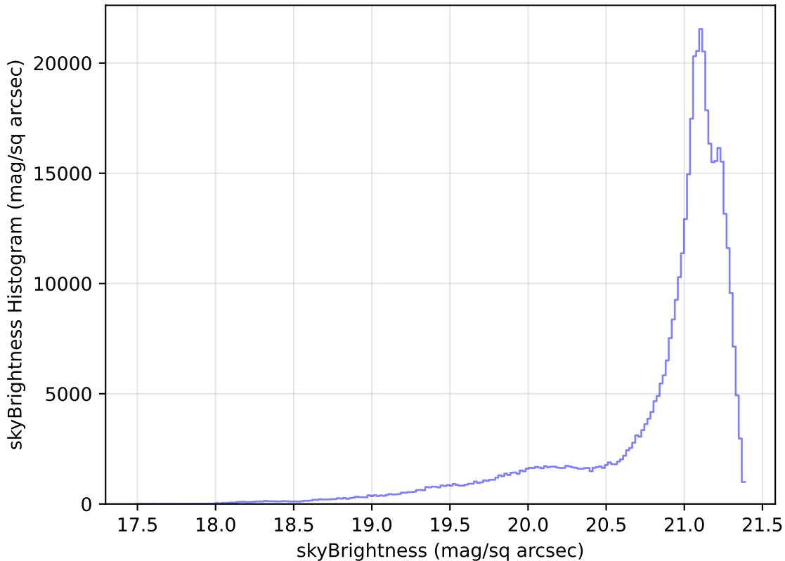
roll_pause_mjdp180_v3.4_10yrs WFD r band: skyBrightness Histogram
