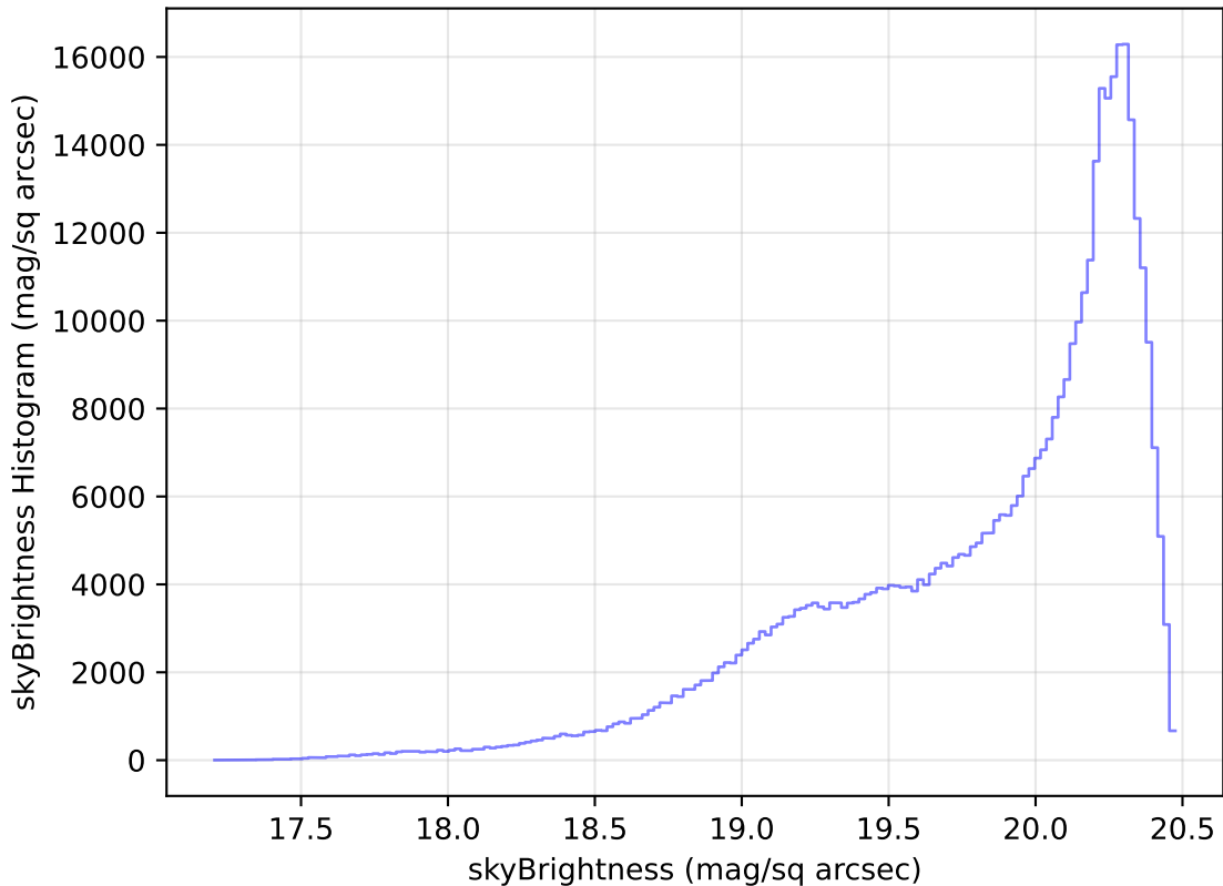
roll_pause_mjdp180_v3.4_10yrs WFD i band: skyBrightness Histogram
