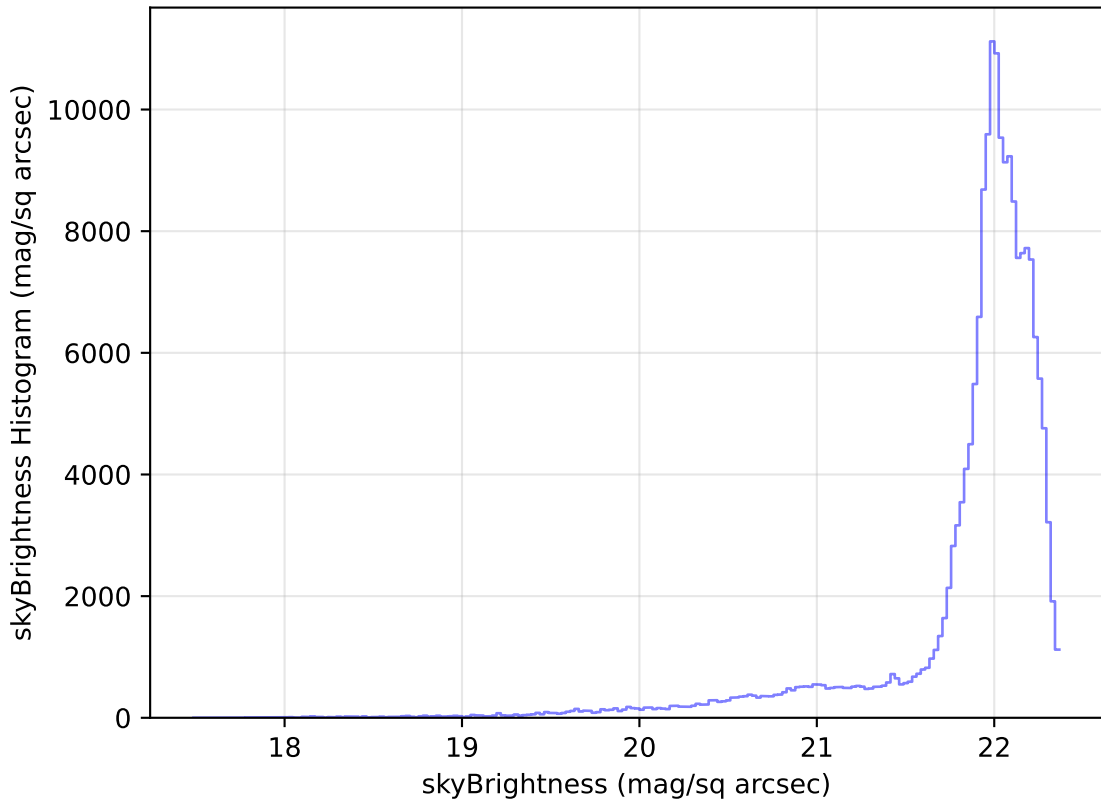
roll_pause_mjdp180_v3.4_10yrs WFD g band: skyBrightness Histogram
