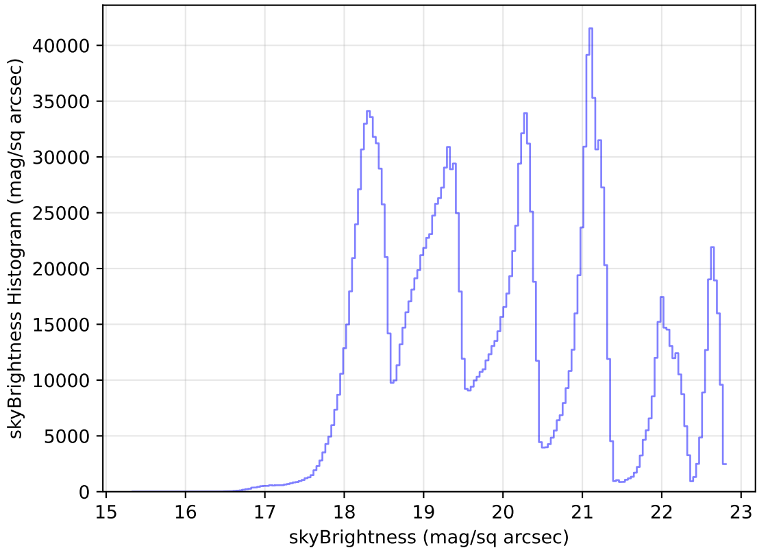
roll_pause_mjdp180_v3.4_10yrs WFD all bands: skyBrightness Histogram
