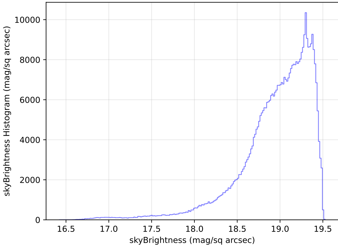
roll_pause_mjdp180_v3.4_10yrs All sky z band: skyBrightness Histogram
