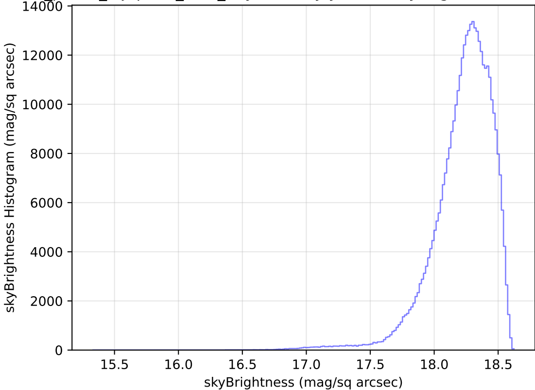
roll_pause_mjdp180_v3.4_10yrs All sky y band: skyBrightness Histogram
