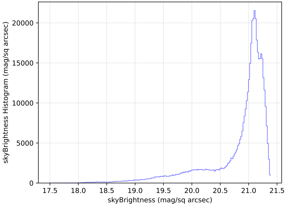
roll_pause_mjdp180_v3.4_10yrs All sky r band: skyBrightness Histogram
