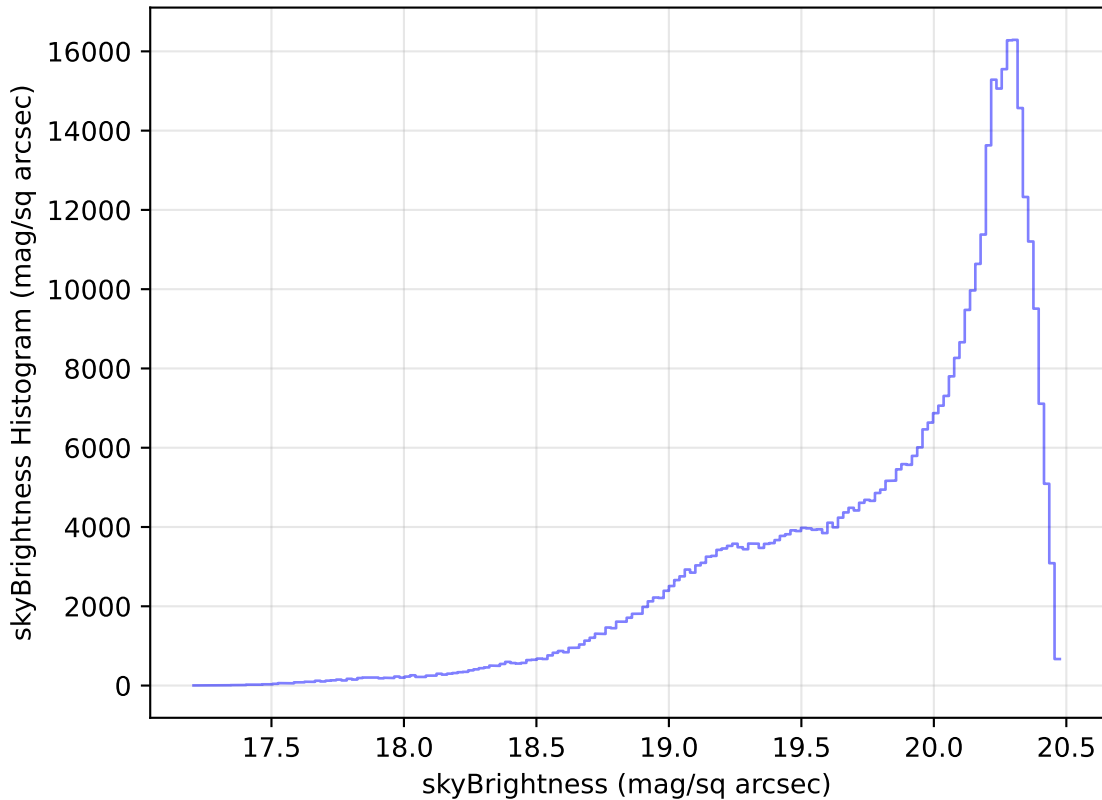
roll_pause_mjdp180_v3.4_10yrs All sky i band: skyBrightness Histogram
