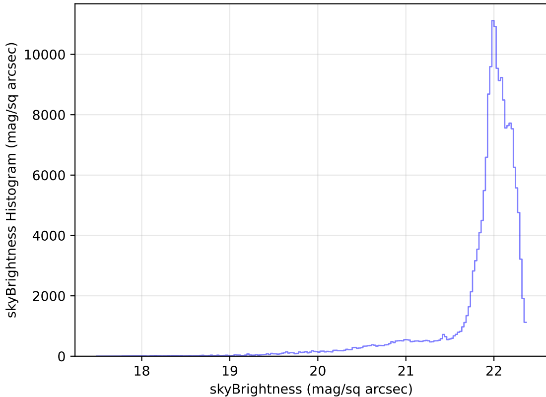
roll_pause_mjdp180_v3.4_10yrs All sky g band: skyBrightness Histogram
