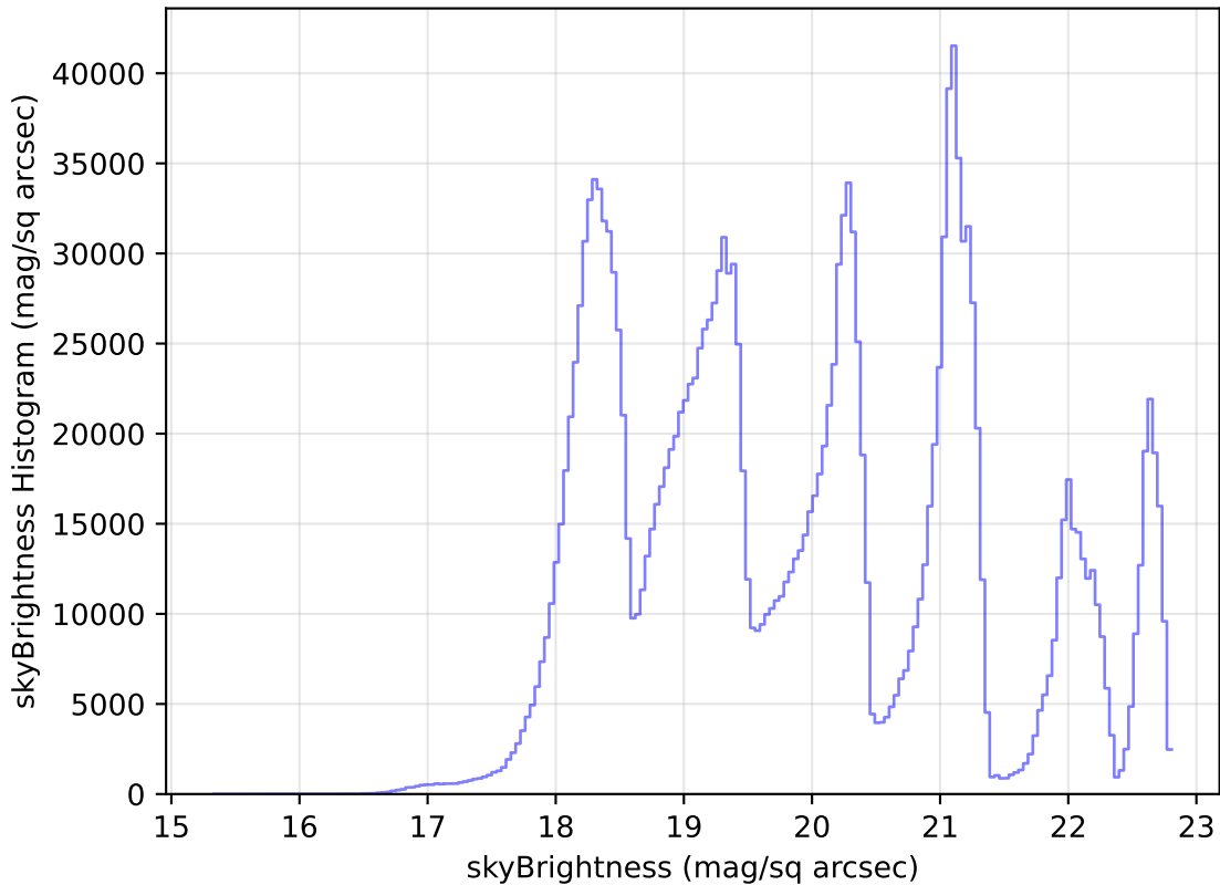
roll_pause_mjdp180_v3.4_10yrs All sky all bands: skyBrightness Histogram
