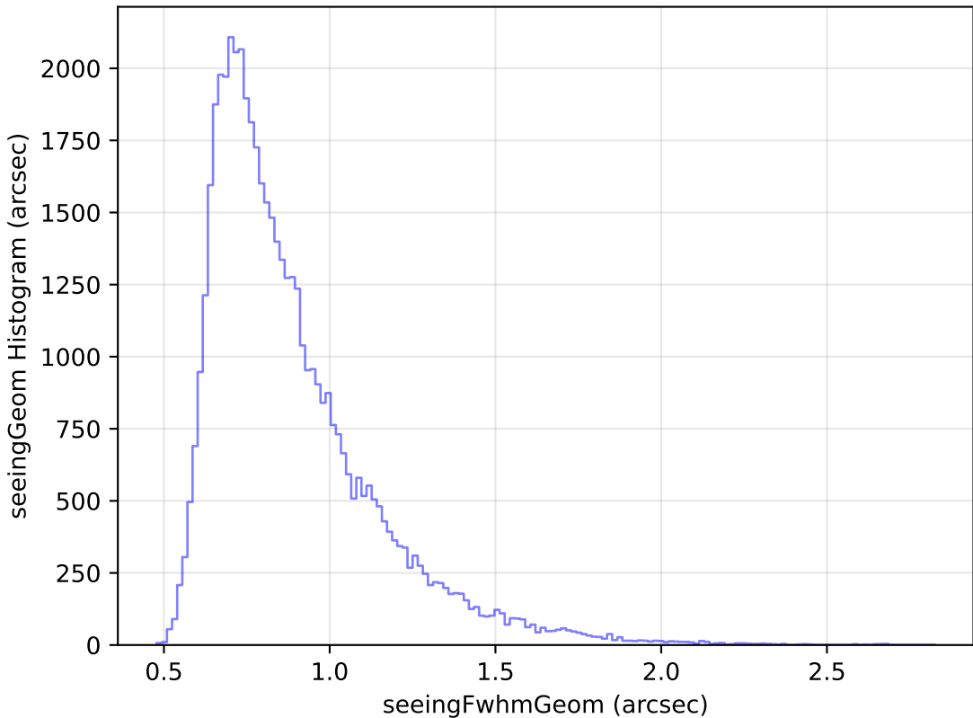
roll_pause_mjdp180_v3.4_10yrs Yr 1 i band: seeingGeom Histogram
