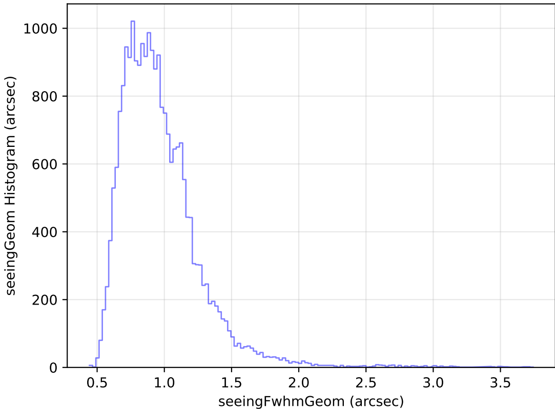
roll_pause_mjdp180_v3.4_10yrs Yr 1 g band: seeingGeom Histogram
