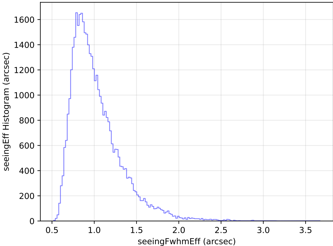
roll_pause_mjdp180_v3.4_10yrs Yr 1 z band: seeingEff Histogram
