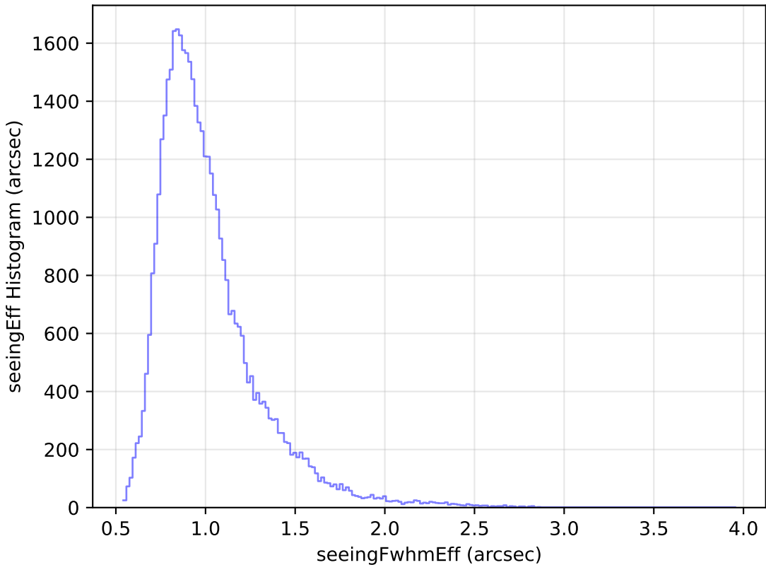
roll_pause_mjdp180_v3.4_10yrs Yr 1 y band: seeingEff Histogram
