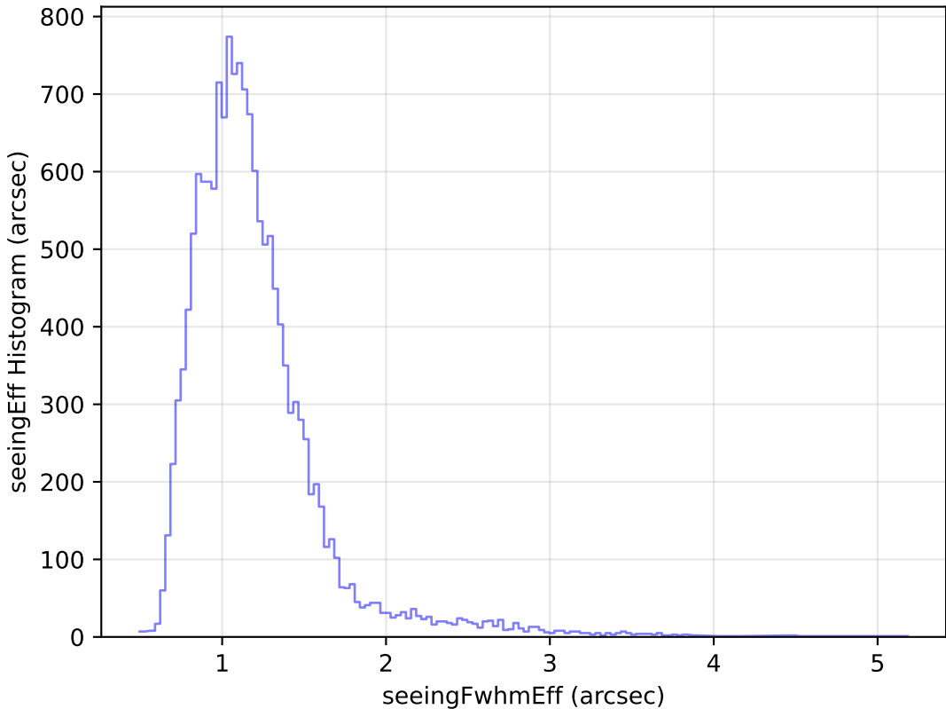
roll_pause_mjdp180_v3.4_10yrs Yr 1 u band: seeingEff Histogram
