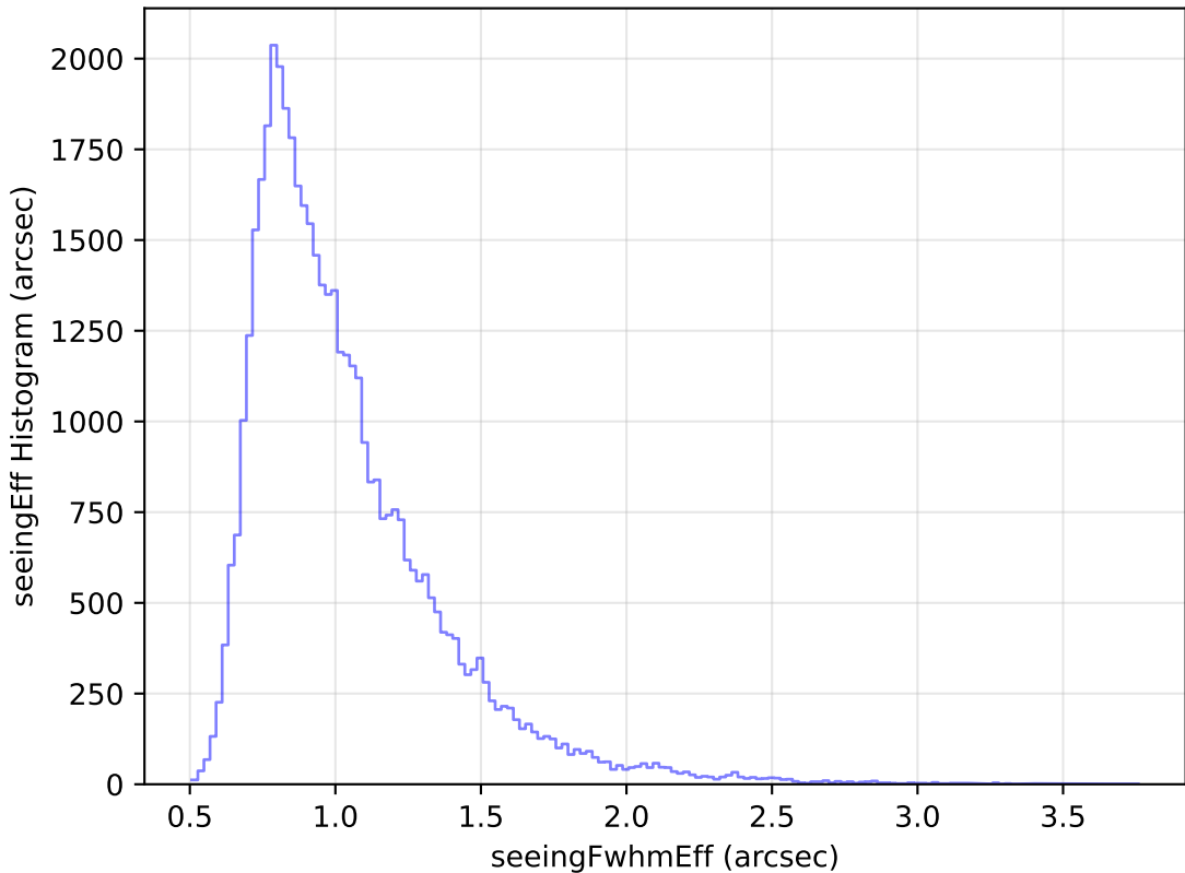
roll_pause_mjdp180_v3.4_10yrs Yr 1 r band: seeingEff Histogram
