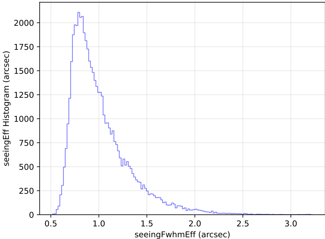
roll_pause_mjdp180_v3.4_10yrs Yr 1 i band: seeingEff Histogram
