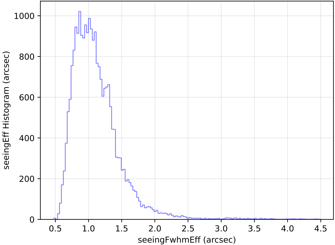
roll_pause_mjdp180_v3.4_10yrs Yr 1 g band: seeingEff Histogram
