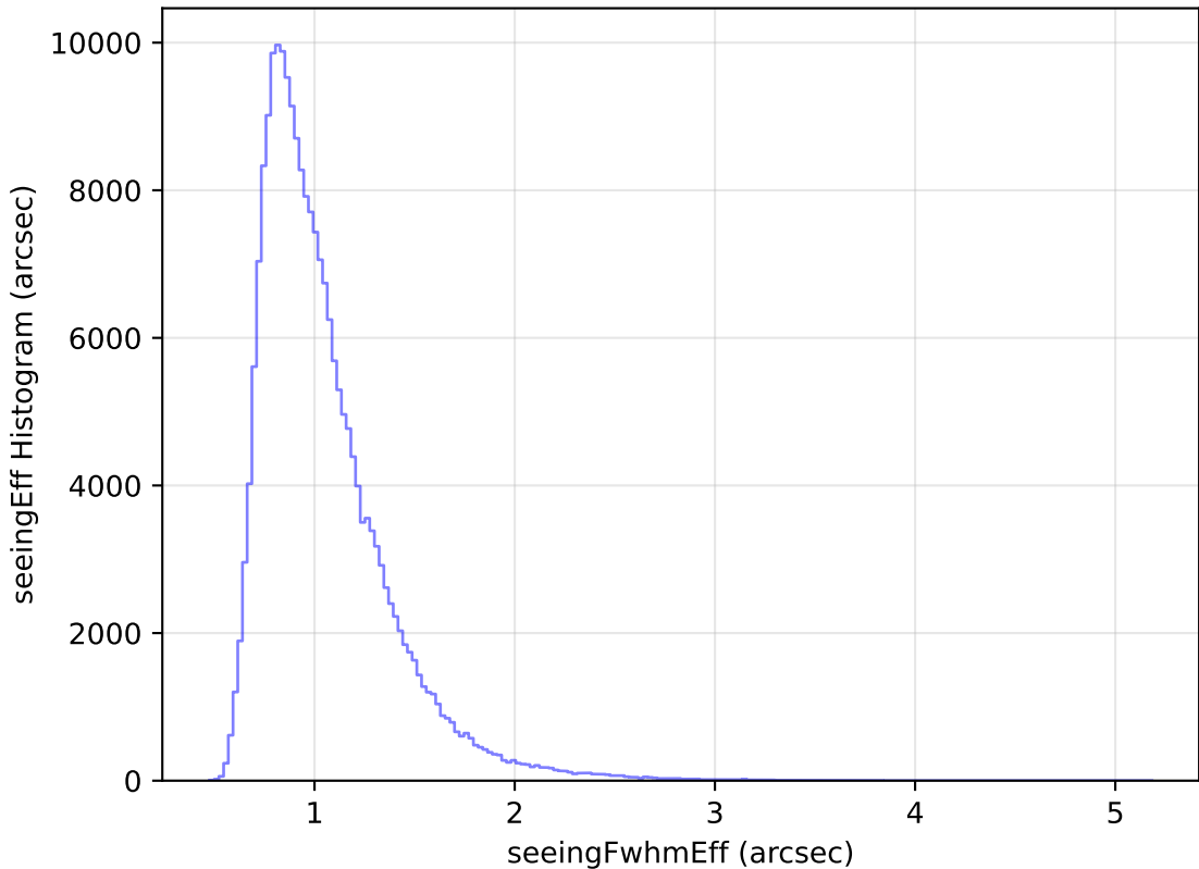
roll_pause_mjdp180_v3.4_10yrs Yr 1 all bands: seeingEff Histogram
