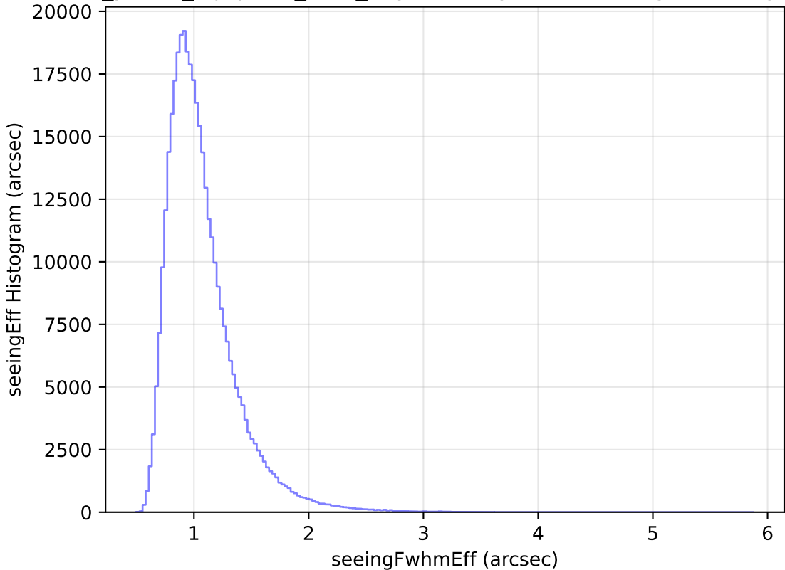
roll_pause_mjdp180_v3.4_10yrs WFD y band: seeingEff Histogram
