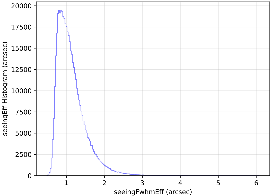
roll_pause_mjdp180_v3.4_10yrs WFD r band: seeingEff Histogram
