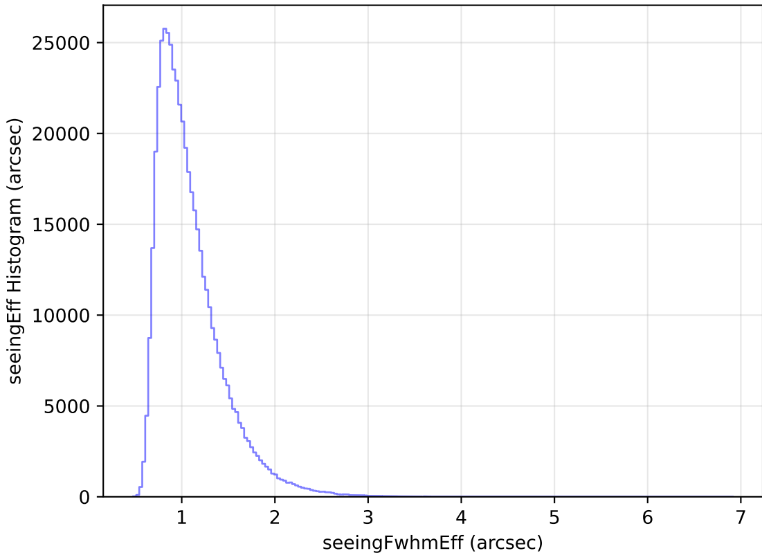
roll_pause_mjdp180_v3.4_10yrs WFD i band: seeingEff Histogram
