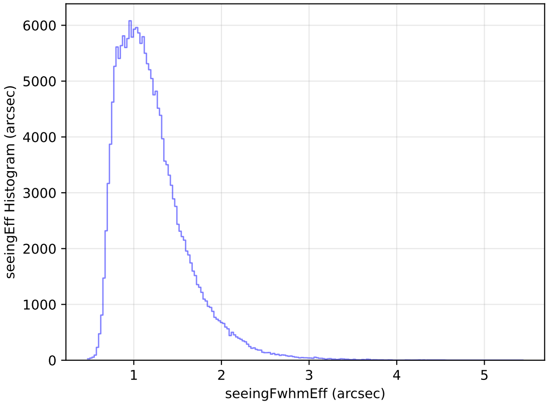
roll_pause_mjdp180_v3.4_10yrs WFD g band: seeingEff Histogram
