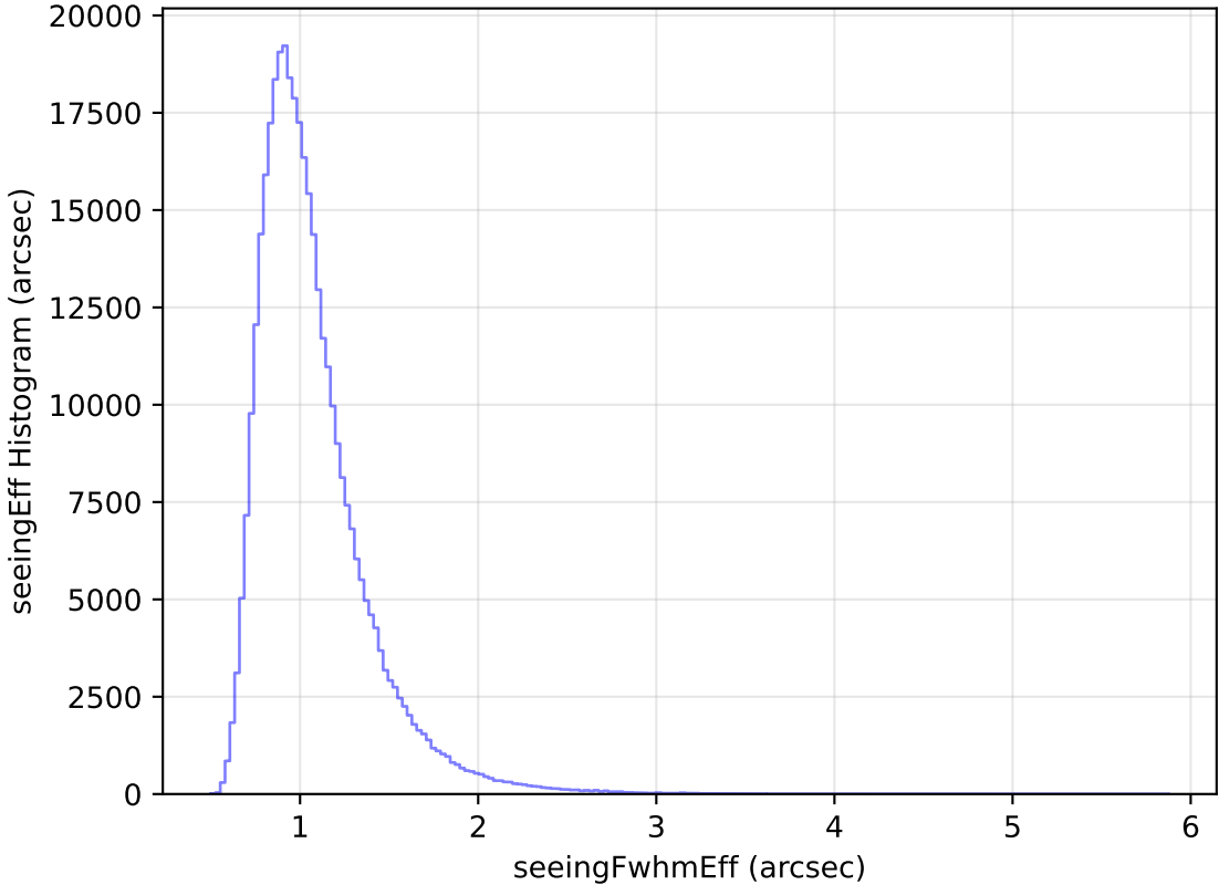
roll_pause_mjdp180_v3.4_10yrs All sky y band: seeingEff Histogram
