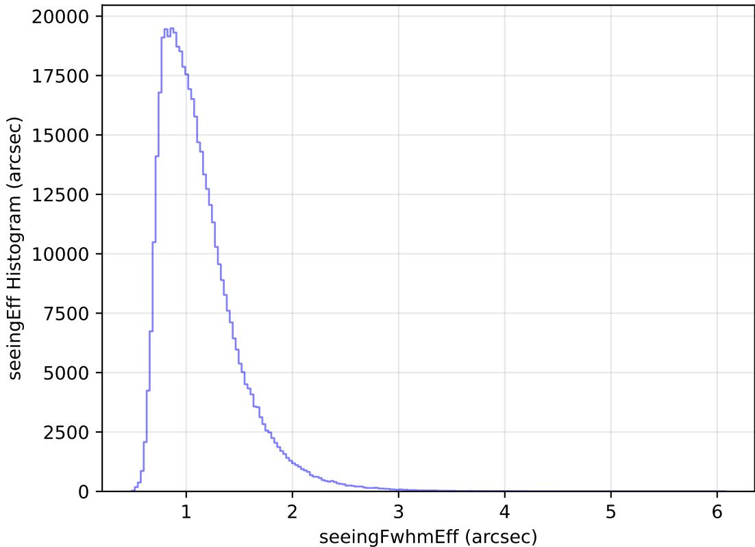
roll_pause_mjdp180_v3.4_10yrs All sky r band: seeingEff Histogram
