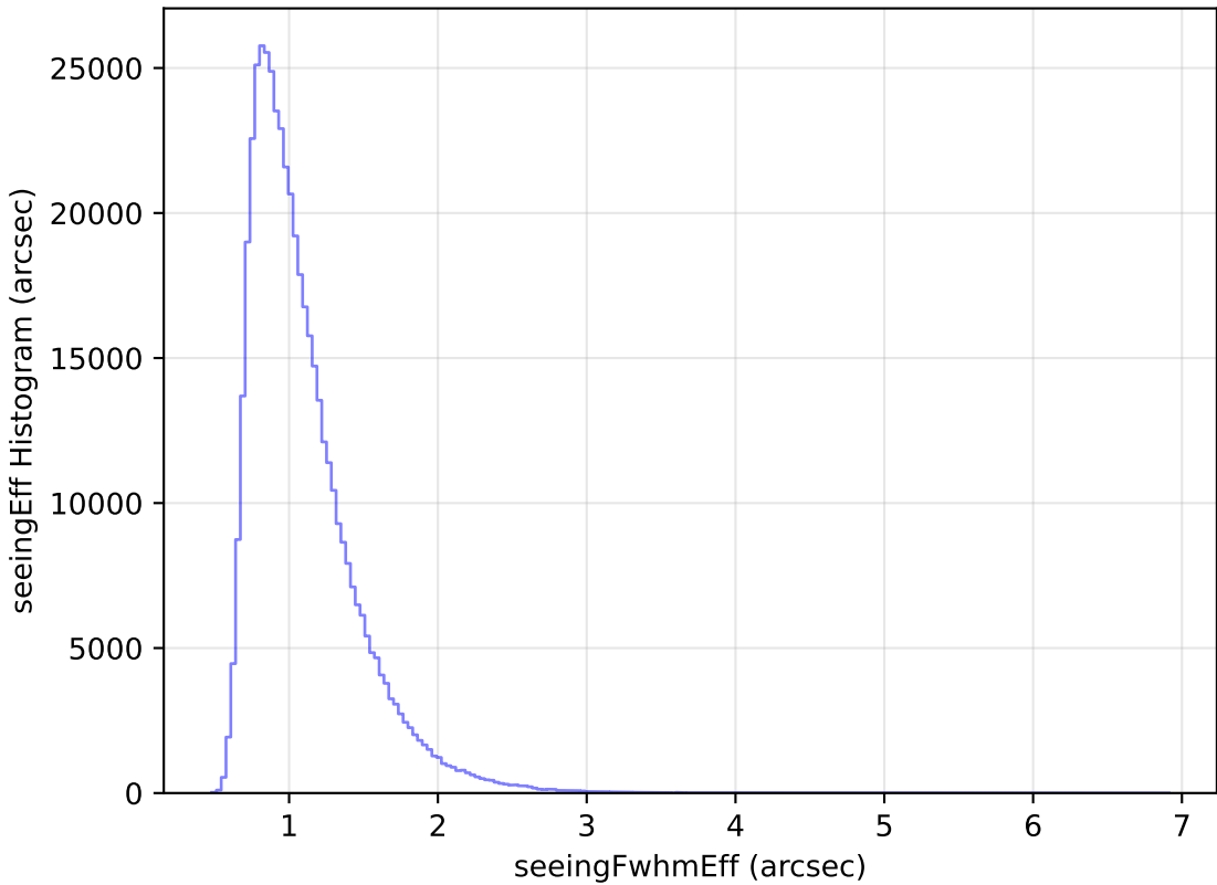
roll_pause_mjdp180_v3.4_10yrs All sky i band: seeingEff Histogram
