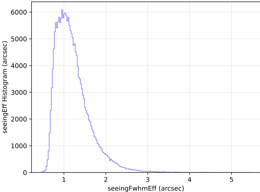
roll_pause_mjdp180_v3.4_10yrs All sky g band: seeingEff Histogram
