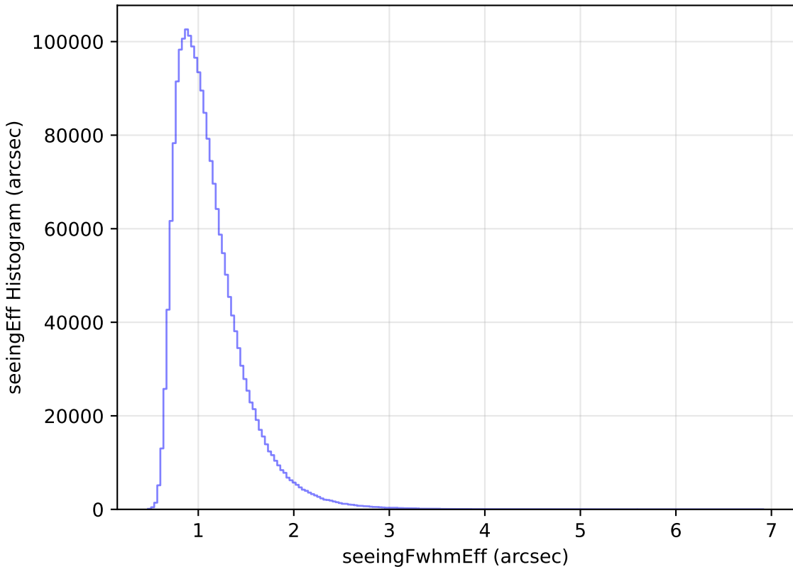
roll_pause_mjdp180_v3.4_10yrs All sky all bands: seeingEff Histogram
