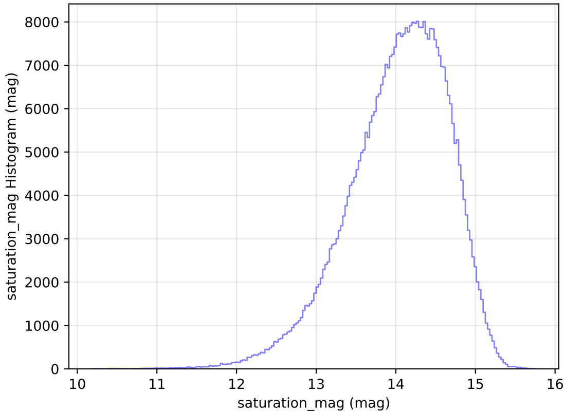
roll_pause_mjdp180_v3.4_10yrs WFD z band: saturation_mag Histogram
