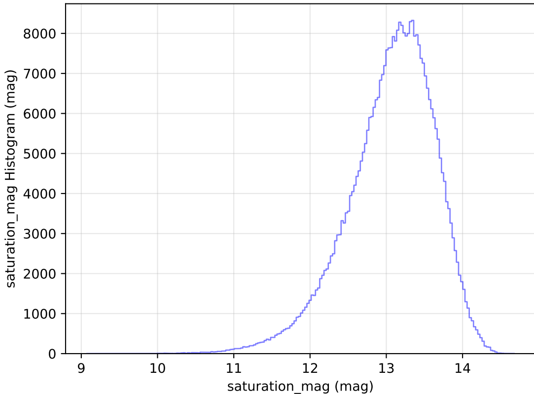
roll_pause_mjdp180_v3.4_10yrs WFD y band: saturation_mag Histogram
