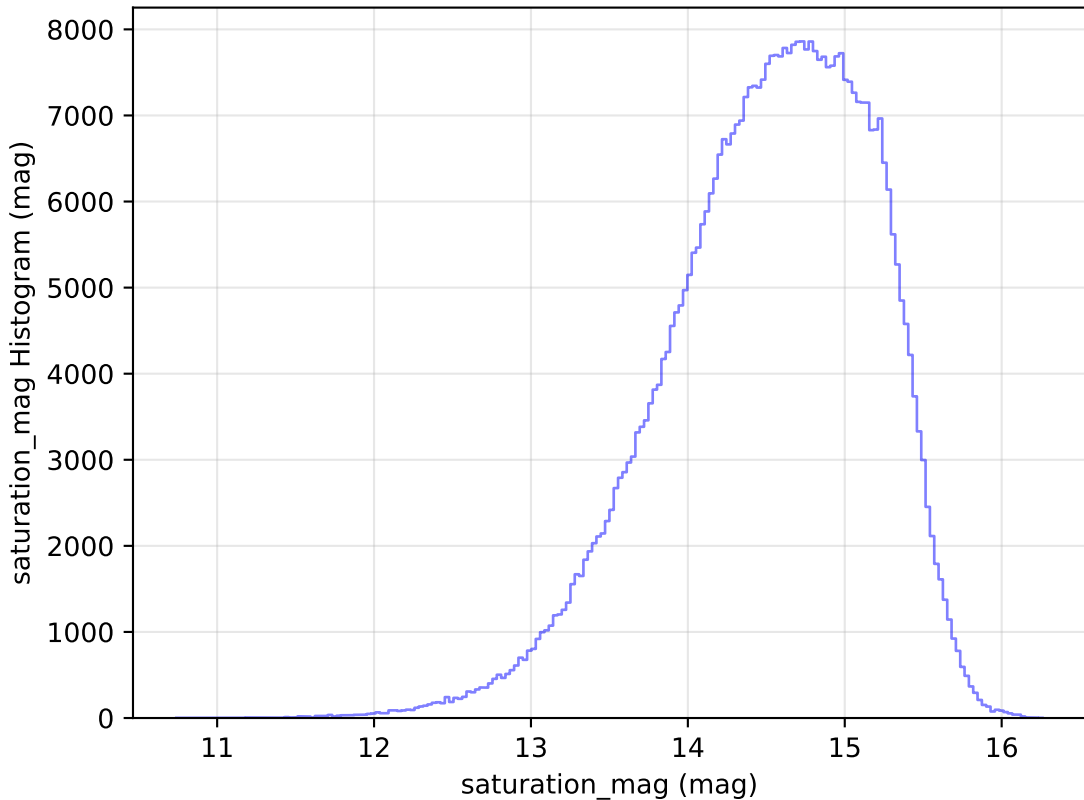
roll_pause_mjdp180_v3.4_10yrs WFD r band: saturation_mag Histogram
