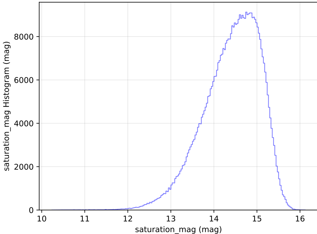
roll_pause_mjdp180_v3.4_10yrs WFD i band: saturation_mag Histogram
