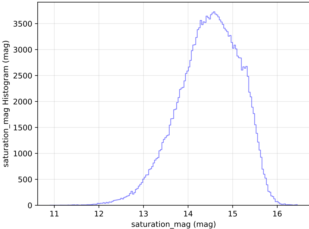
roll_pause_mjdp180_v3.4_10yrs WFD g band: saturation_mag Histogram
