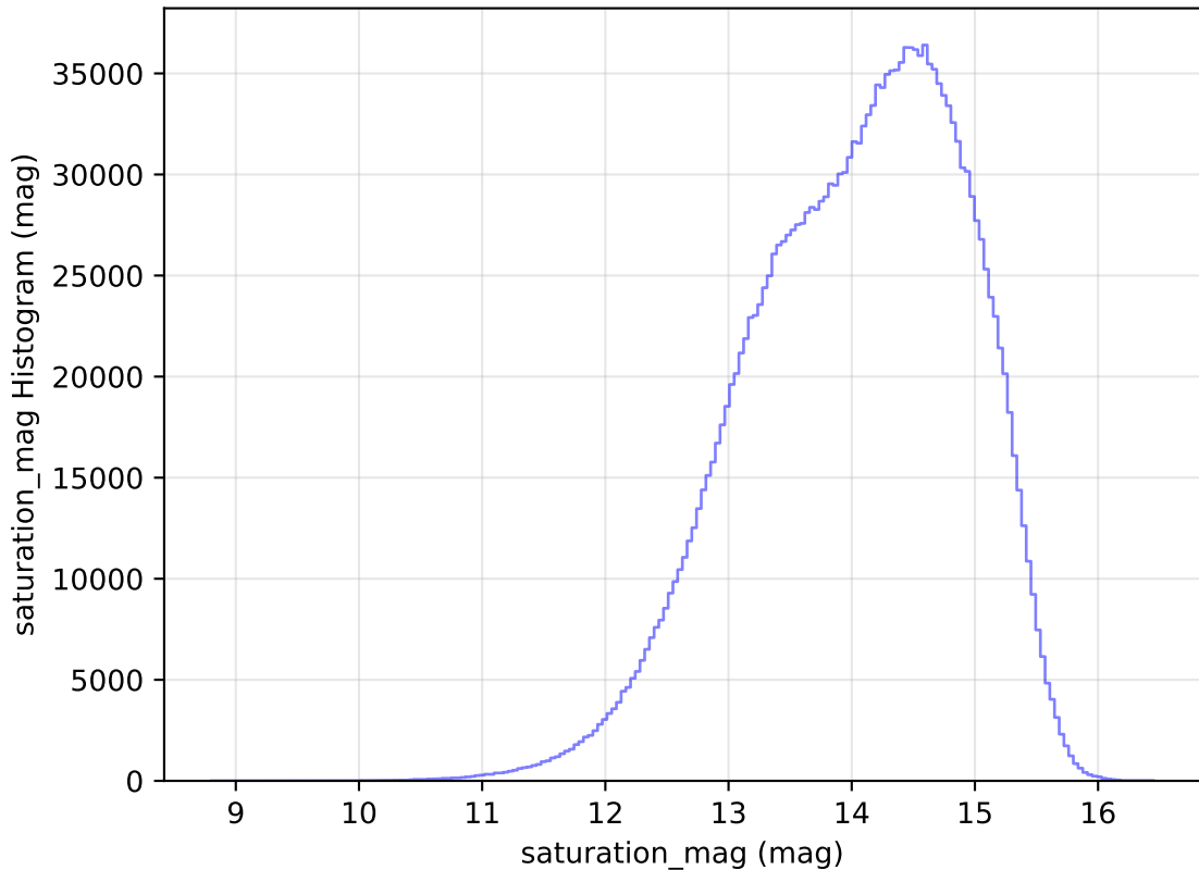
roll_pause_mjdp180_v3.4_10yrs WFD all bands: saturation_mag Histogram
