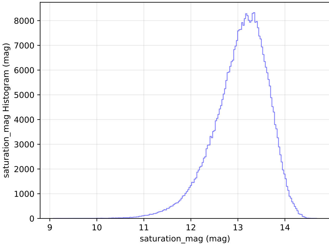
roll_pause_mjdp180_v3.4_10yrs All sky y band: saturation_mag Histogram
