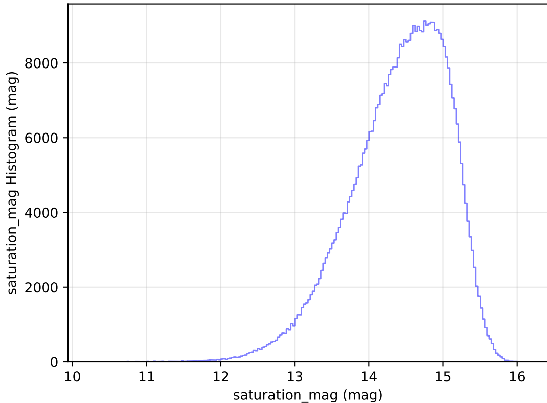
roll_pause_mjdp180_v3.4_10yrs All sky i band: saturation_mag Histogram
